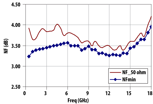
Figure 6. Noise Figure (Vc = 1.8 V)
