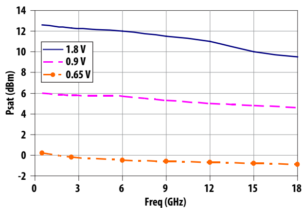
Figure 9. Saturated Power
