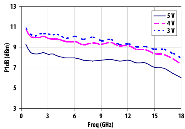
Figure 16. Output P1dB over Vdd
