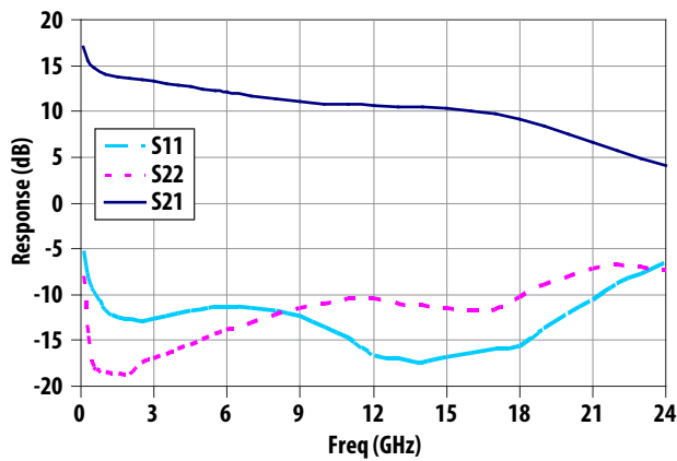
Figure 5. Broadband Gain and Return Losses (Vc = 1.8 V)
