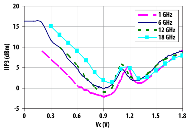
Figure 8. Input IP3 vs. Vc
