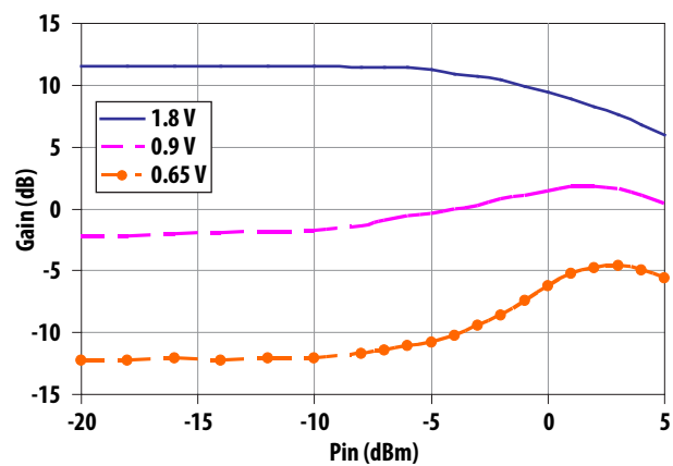
Figure 10. Gain vs. Pin at 6 GHz
