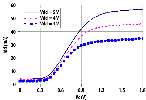
Figure 12. Supply Current over Bias
