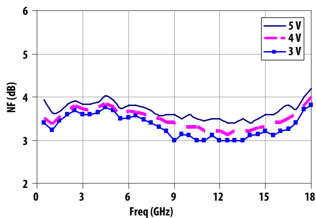
Figure 14. Noise Figure over Vdd
